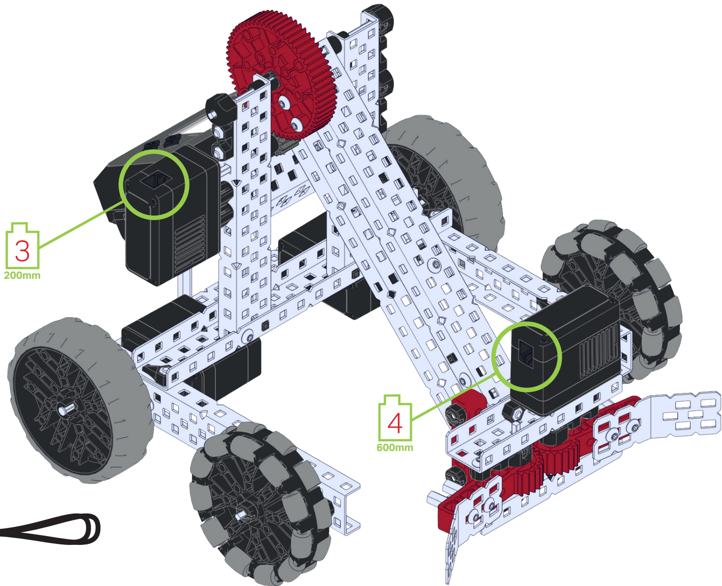
1x 200mm Smart Cable
